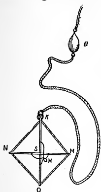
DIAGRAM OF FLOAT- ING ANCHOR.
